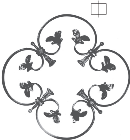
R 24/B/1 ▧ 12×6 mm Ø 460 mm
