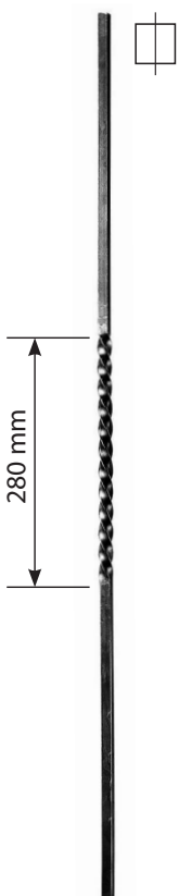
R 1148/5 □ 12×12 mm H 1000 mm
