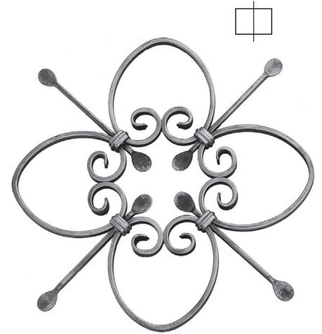
R 1009/2 ▧ 12×6 mm Ø 370 mm
