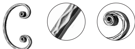
R 1296/7 \square 12×6 mm 90×140 mm
