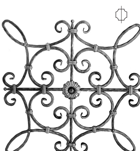
R 480/1 □ 12×12 mm 660×660 mm
