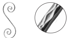
R 641/8 \square 12×6 mm 120×360 mm
