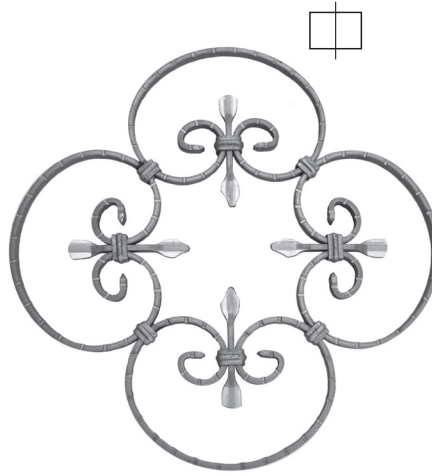
R 24/1 ▧ 10×5 mm Ø 380 mm
