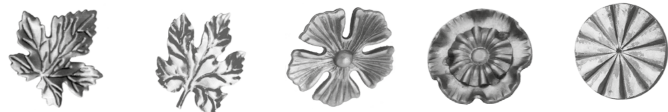
R 138/11 \sphericalangle 0,5 mm 75×70 mm R 138/12 \sphericalangle 0,5 mm 95×105 mm R 138/14 \sphericalangle 4 mm \varnothing 120 mm R 138/15 \sphericalangle 2 mm \varnothing 60 mm R 654/5 \sphericalangle 6 mm \varnothing 60 mm
