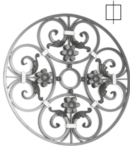
R 24/E/1 □ 12×12 mm ∅ 600 mm
