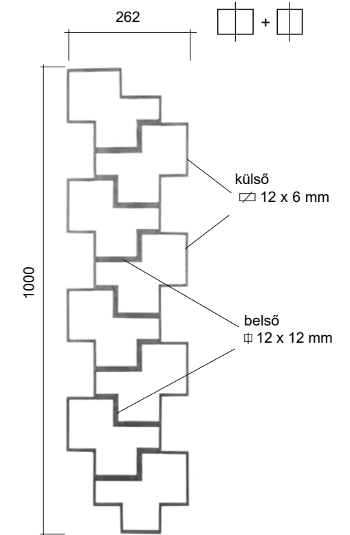
RGD 293/1 □ 12x6 mm + □ 12 mm 1000x262 mm
