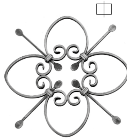
R 1009/2 □ 12×6 mm ∅ 370 mm
